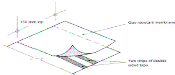
Figure 11: Sealing joints in the radon barrier
