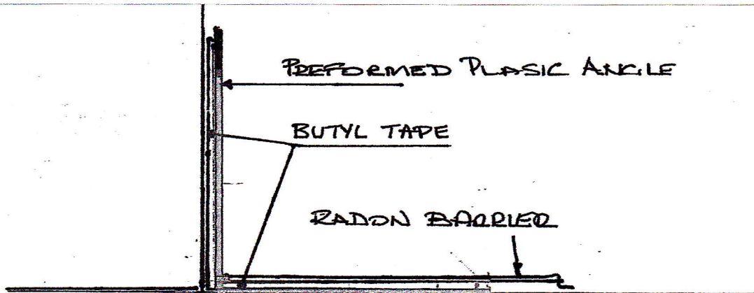
FULL SIZE SECTION OF ANGLE & TAPE
