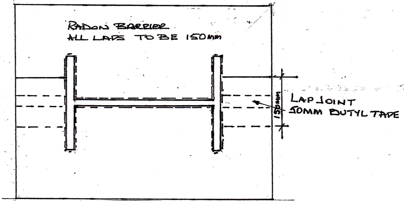
FULL SIZE SECTION OF ANGLE & TAPE
